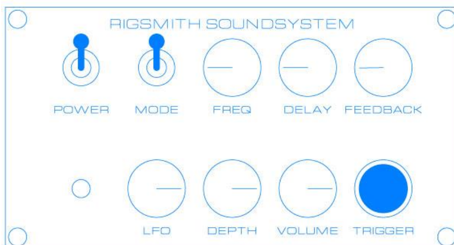
Figure 1: RS1 DESKTOP TOP PANEL
